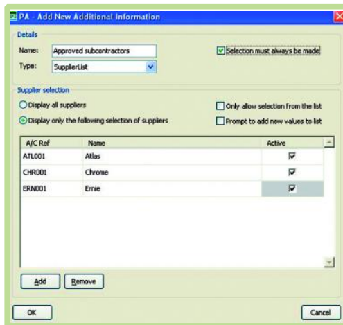
Screenshot 2: User-defined additional analysis fields – showing 200-data types and mandatory user options.
